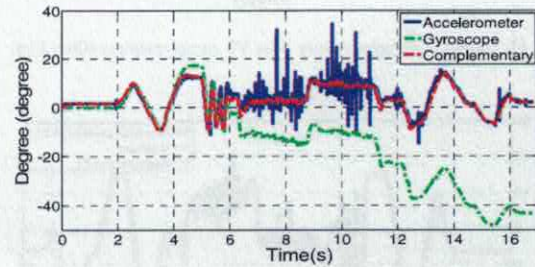
Fig. 10. Output of complementary filter
