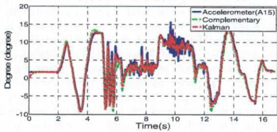
Fig. 13, Output of complementary Filter VS Kalman filter
