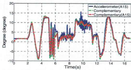
Fig. 11, Output of complementary filter VS complementary filter(A15)
