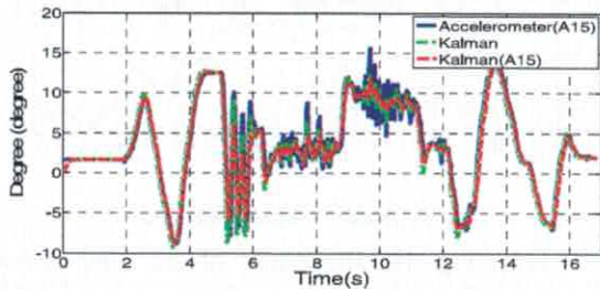
Fig. 12, Output of Kalman filter VS Kalman filter (A15)
