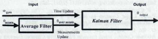
Fig. 8. Average filter using on Kalman Filter
