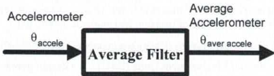
Fig. 3, Average filter
