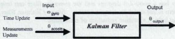
Fig 7. Kalman Filter
