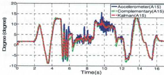
Fig. 14, Output of complementary filter(A15) VS Kalman filter(A15)
